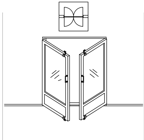
Figure 17 Double swing doors
