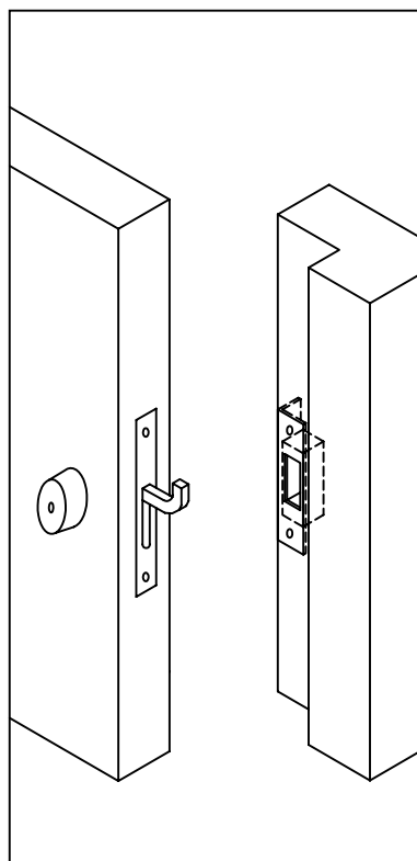
Figure 19 Security lock
